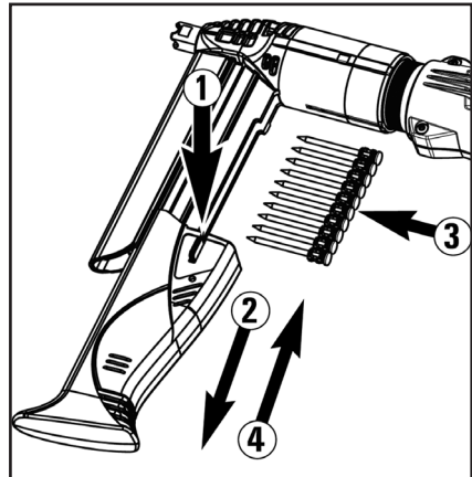
1b. TOOL FITTED WITH FASTENER MAGAZINE
